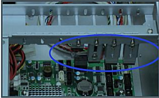
↑ Captive Bolt for tool-free design
